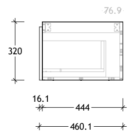
End View (1000, 1200, 1400)
